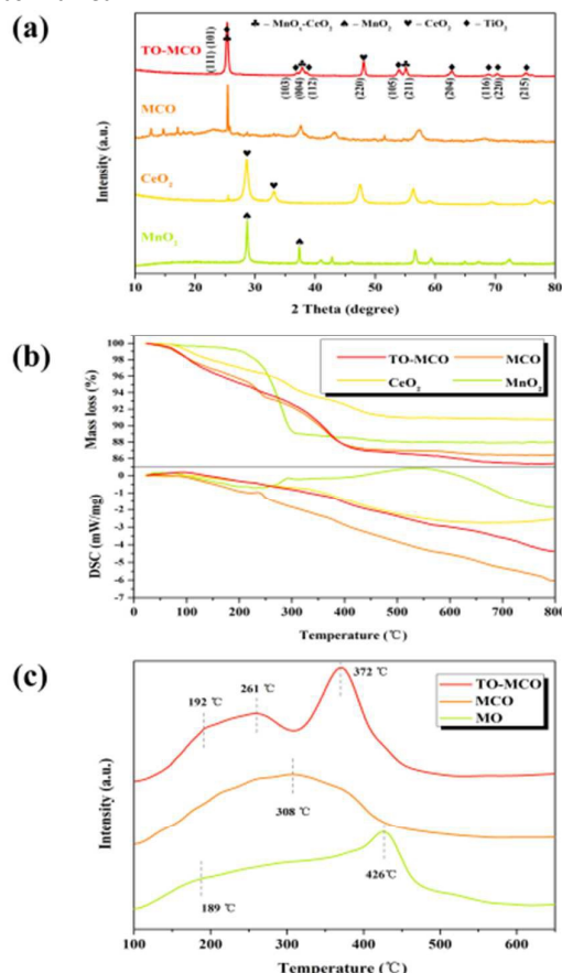
Fig. 1 XRD patterns of MnO 2 , CeO 2 , MCO, and TO-MCO catalyst (a); thermogravimetry differential scanning calorimetry profiles of the as-prepared catalysts (b); H 2 -TPR profiles of the as-prepared catalysts (c).
