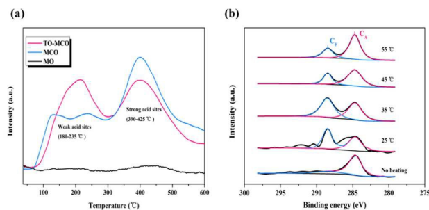
Fig. 5 NH 3 -TPD profiles of the as-prepared catalysts (a) and in situ C 1s XP spectra of the HCHO-exposed TO-MCO under heating Ar (b).
